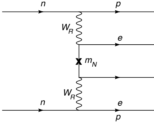
Figure 4: Neutrinoless double \beta decay through W_R and N
