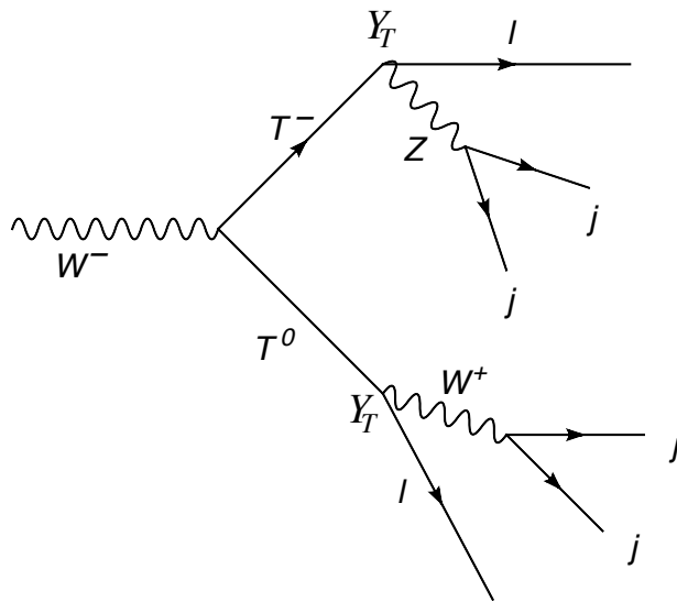
Figure 7: The same sign dilepton signature of type III seesaw through the production of the charged and neutral components of a fermion triplet T_F
