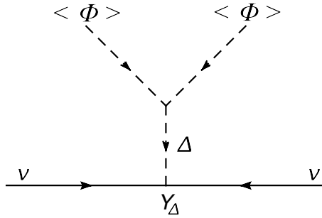
Figure 3: Diagrammatic representation of the Type II see-saw
