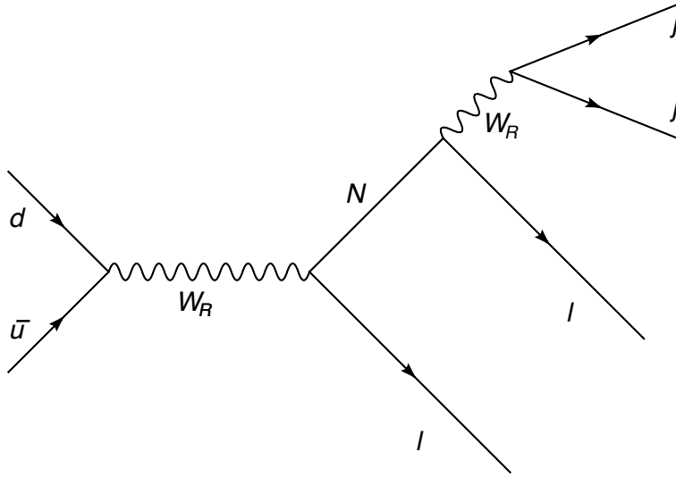
Figure 5: Production of lepton number violating same sign dileptons at colliders through W_R and N
