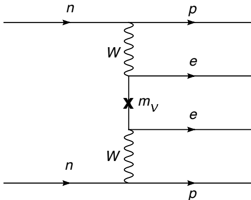
Figure 1: Neutrinoless double \beta decay through a Majorana mass m_M which breaks a neutrino fermionic line
