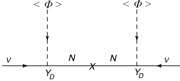
Figure 2: Diagrammatic representation of the Type I see-saw
