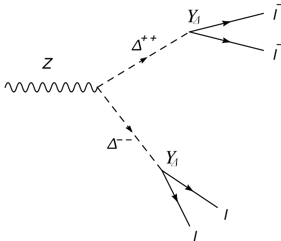
Figure 6: Production of a pair of double charged Higgs scalars and subsequent decay into pairs of same sign dileptons
