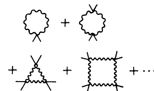
FIG. 4. The photon contribution to the one-loop approximation for the effective potential.
